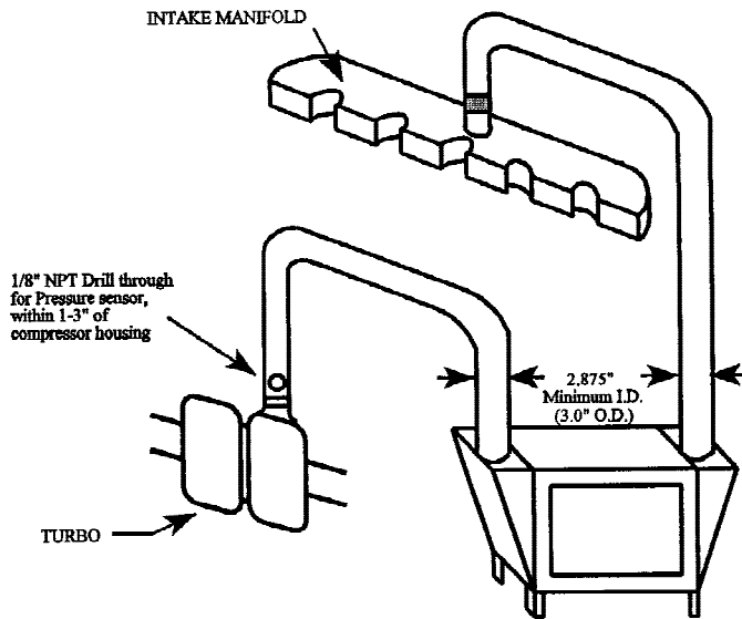
FIG. A2.11 Test Cell Slave Intercooler Arrangement
