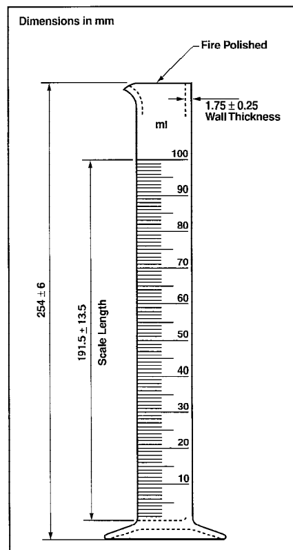
NOTE—1 to 100 mL in 1 mL graduations; tolerance ± 1.0 mL. FIG. A2.3 100 mL Graduated Cylinder
