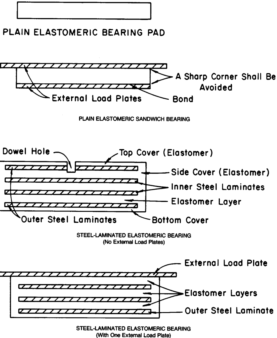
FIG. 1 Examples of the Construction of Elastomeric Bearings
